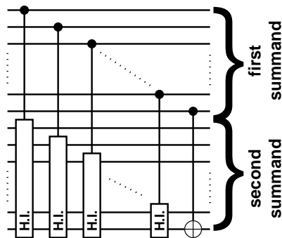
Figure 5. An adder circuit.
