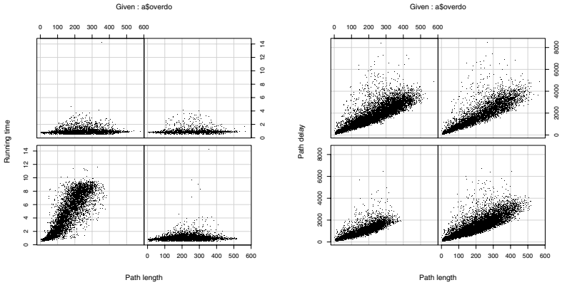
Fig. 4. Running time and path delay against the number of nodes on the path for four different values of overdo (0, 0.15, 0.25, 0.5). The figures correspond to increasing overdo parameters and are to be read row wise and bottom up. Note the steep decrease in running time as we go from overdo = 0 to overdo = .15; the improvement is small after that. We will take a closer look at the horn-shape with overdo = 0, but note that the running time appears linear in the other three plots. In fact, it seems constant , but a linear fit shows a very low slope, as is to be expected. However, the quality of the paths output continues to decay with increased overdo
